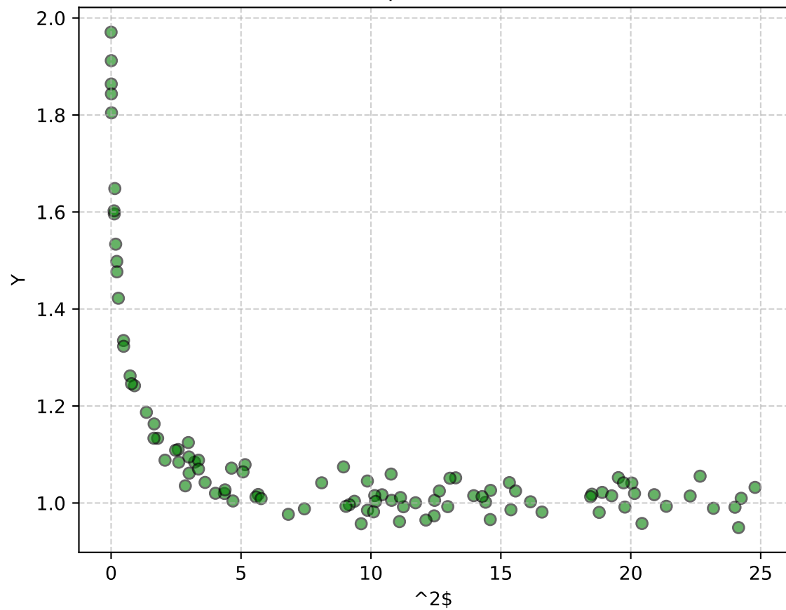
Scatter plot of \hat{2} vs Y
