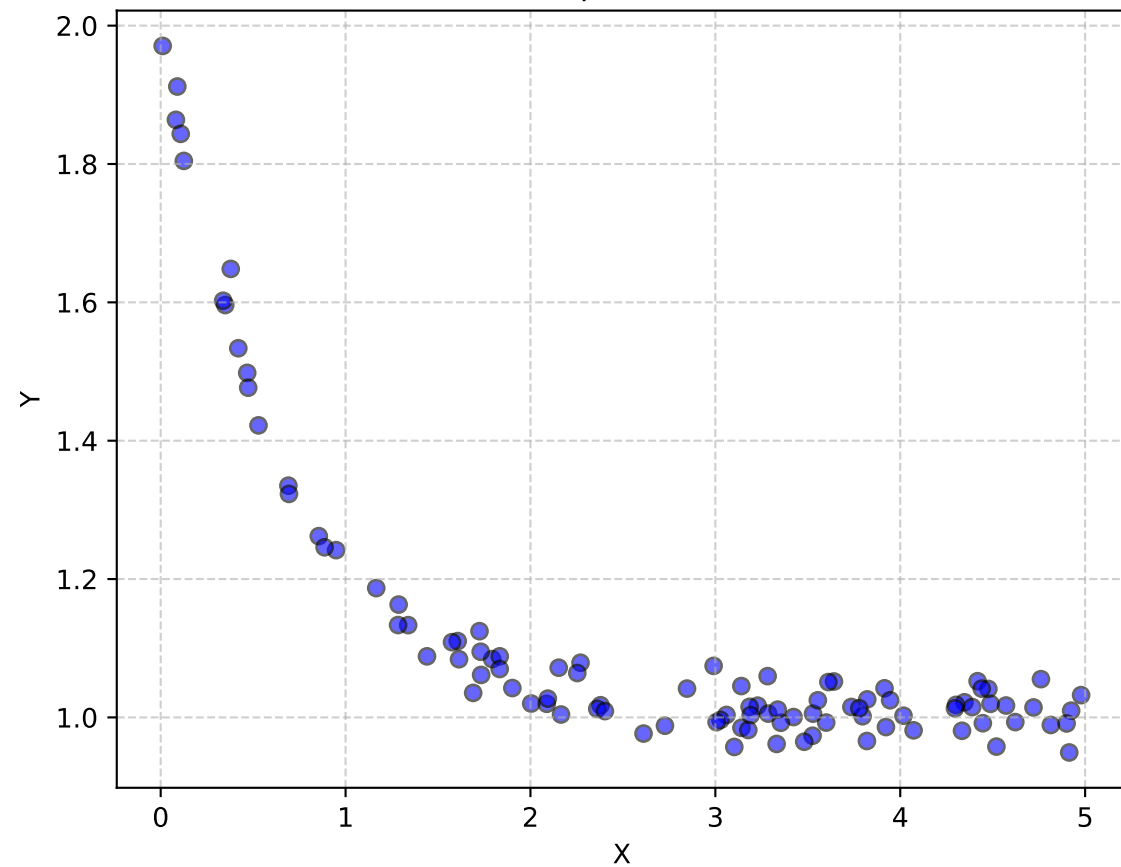
Scatter plot of X vs Y
